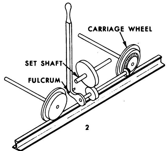
Figure 8-18. Power receders.
